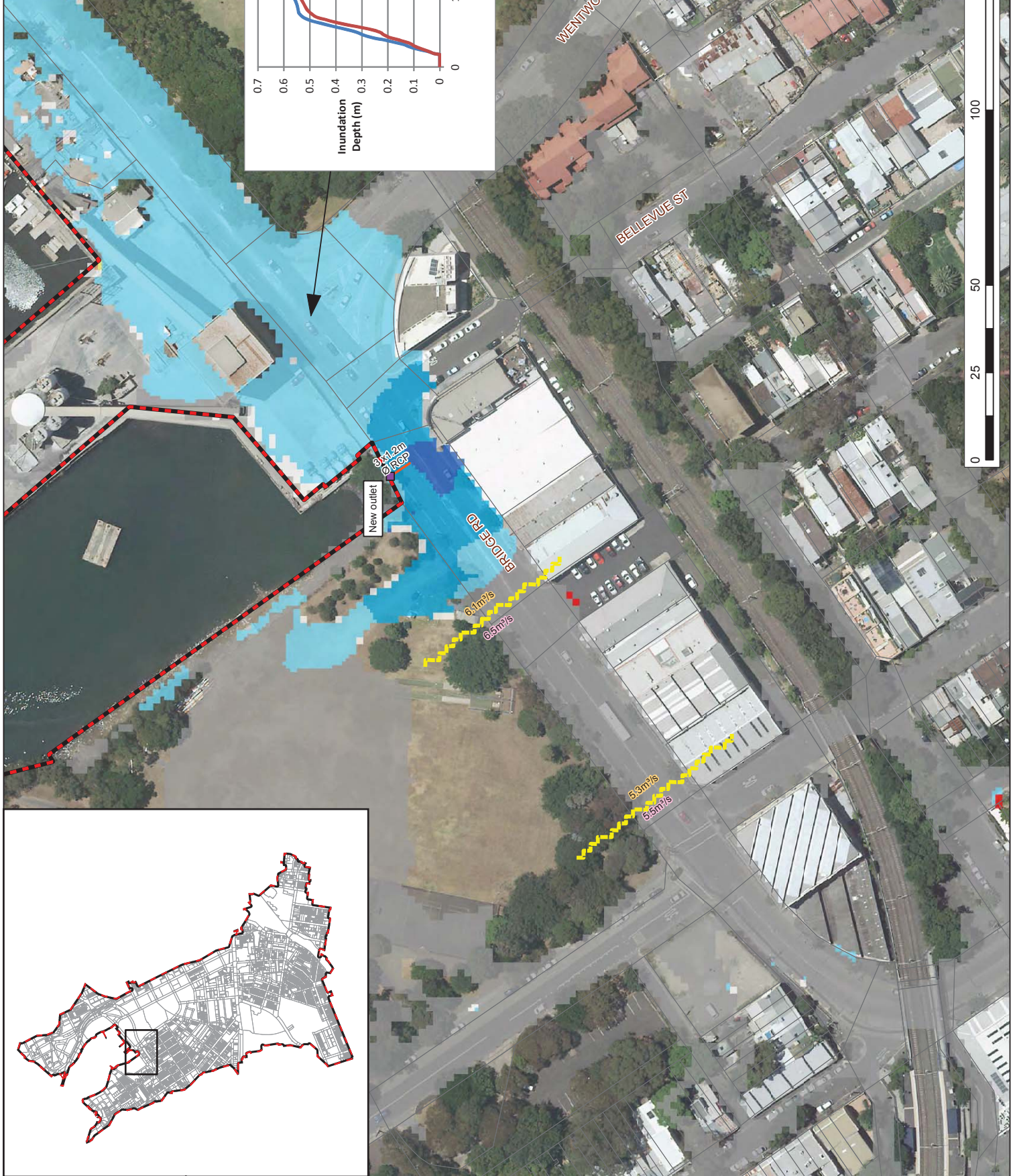
FIGURE 35 OPTION FM - BB03 NEW OUTLET TO BLACKWATTLE BAY FLOOD IMPACT MAP 10% AEP DESIGN FLOOD EVENT
